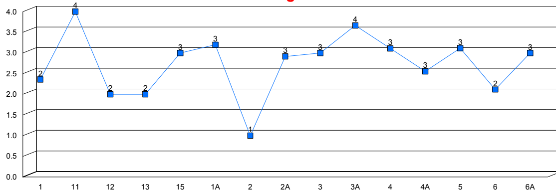
Average Score
