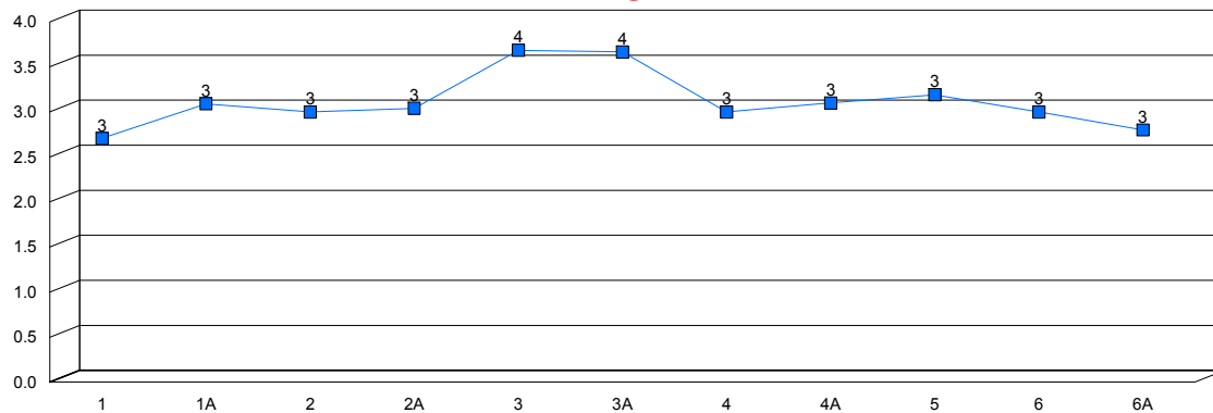
Average Score
