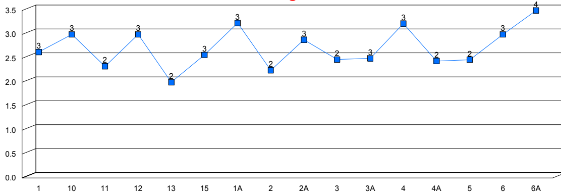
Average Score
