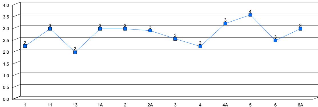
Average Score
