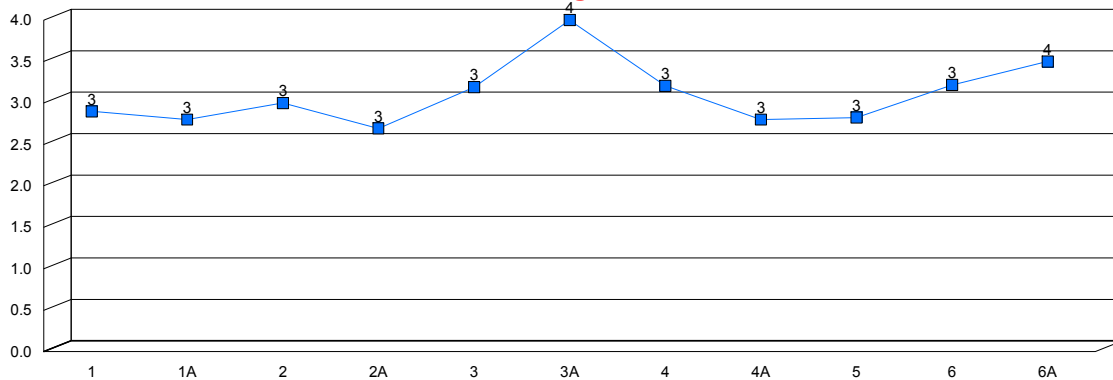
Average Score
